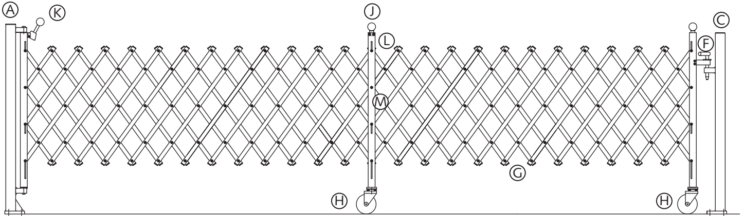
Long gate configuration with Standard Anchor Post, Latch Post and Padlockable Latch Pin and Center Support Stanchion
