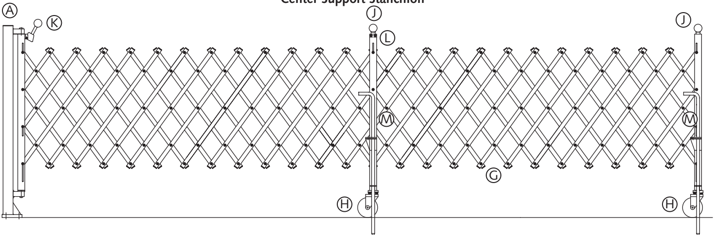
Long gate configuration with Standard Anchor Post, Center Support Stanchion, and Drop Pin anchoring to the floor. NOTE: When Drop-Pin anchoring is in place the 200 lb. OSHA side load requirement is met.
